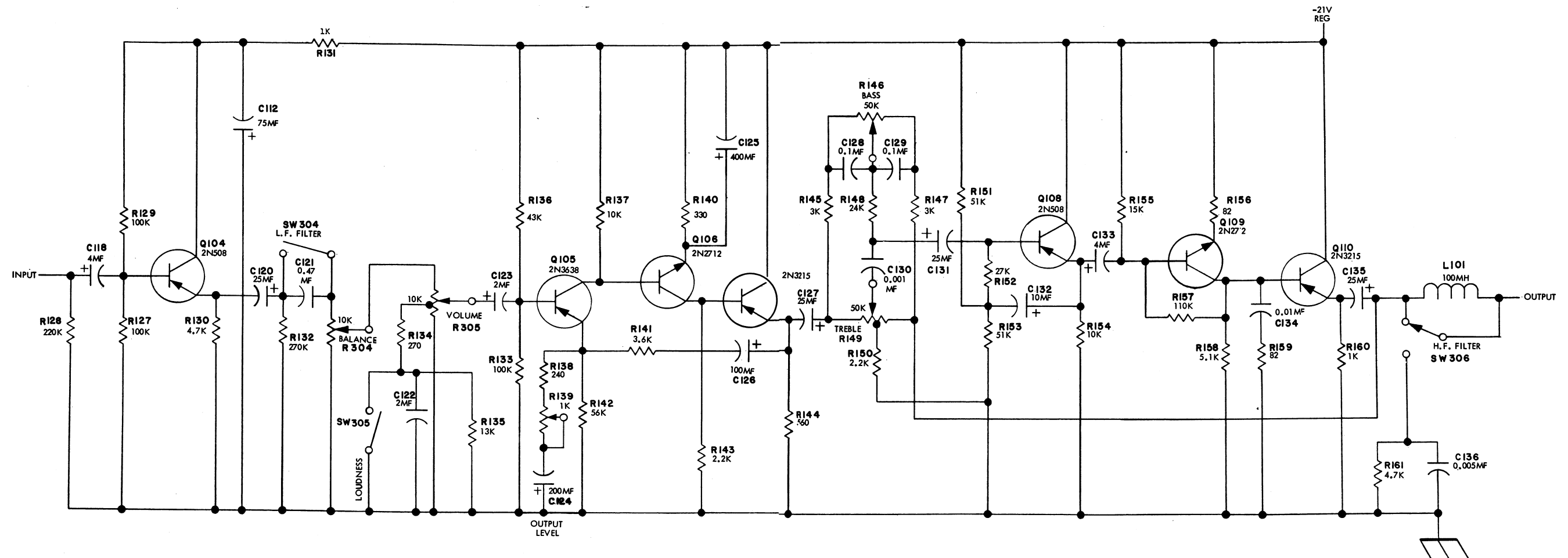
LINE AMPLIFIER
