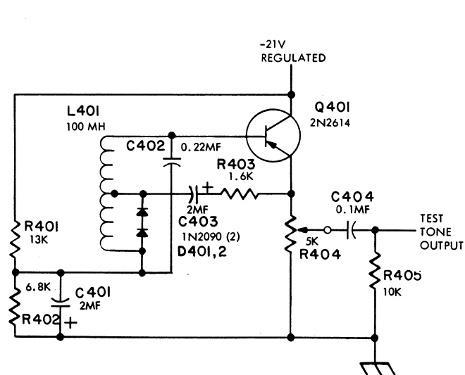
TONE OSCILLATOR
